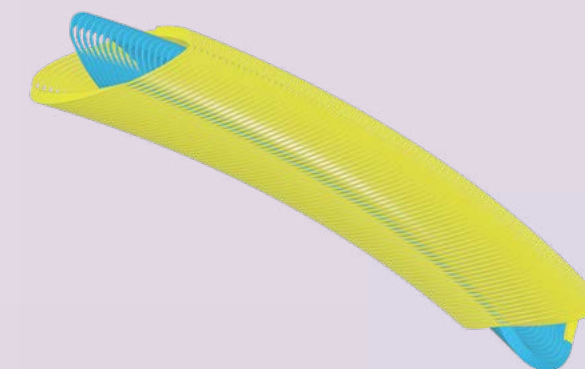
Figure 1: Sketch of a Curved CCT dipole of 4.5 T to which is superimposed a small quadrupole component of 5 T/m. Credit to INFN-Milano-LASA.
