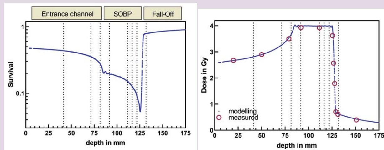
Figure 1: Example for modelling treatment plans using TRIP98. The blue curve represents survival for a SOB geometry of 60x80x40 mm. Dashed lines mark the positioning of the cells for the in vitro experiment, which is supposed to cover entrance channel, SOB and Fall-off. A) Expected survival for the model cell line. B) Corresponding dose-depth-distribution.
